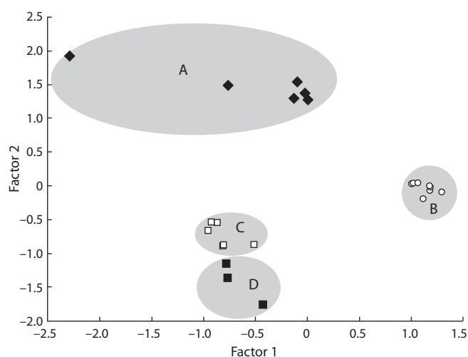
Fig. 3. Results of a factor analysis of alkaloid composition and content in the seeds of the lupine cultivar "Oligarkh" measured under various extraction techniques (A, B, C and D).
