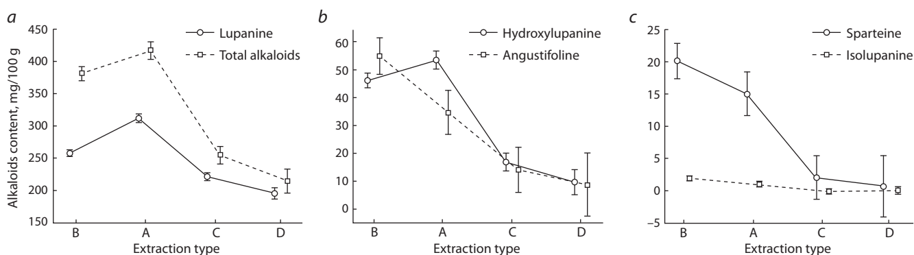
Fig. 2. ANOVA of the content (mg/100 g) of the total alkaloids and lupanine (a), 13-hydroxylupanine and angustifoline (b), sparteine and isolupanine (c) in the seeds of the lupine cultivar "Oligarkh" measured under various extraction techniques (A, B, C and D).
