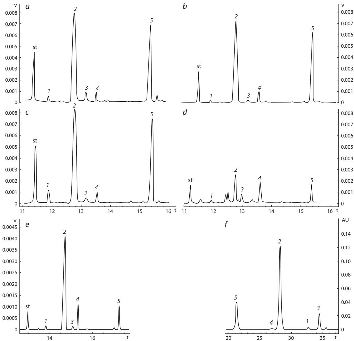
Fig. 1. Chromatograms of the samples: a – A_1 ; b – A_2 ; c – C; d – D; e – B, obtained by GC-MS; f – chromatogram of acid salts of the alkaloids obtained by HPLC-MS. Alkaloids: st – standard; 1 – sparteine; 2 – lupanine; 3 – angustifoline; 4 – isolupanine; 5 – 13-hydroxylupanine.
