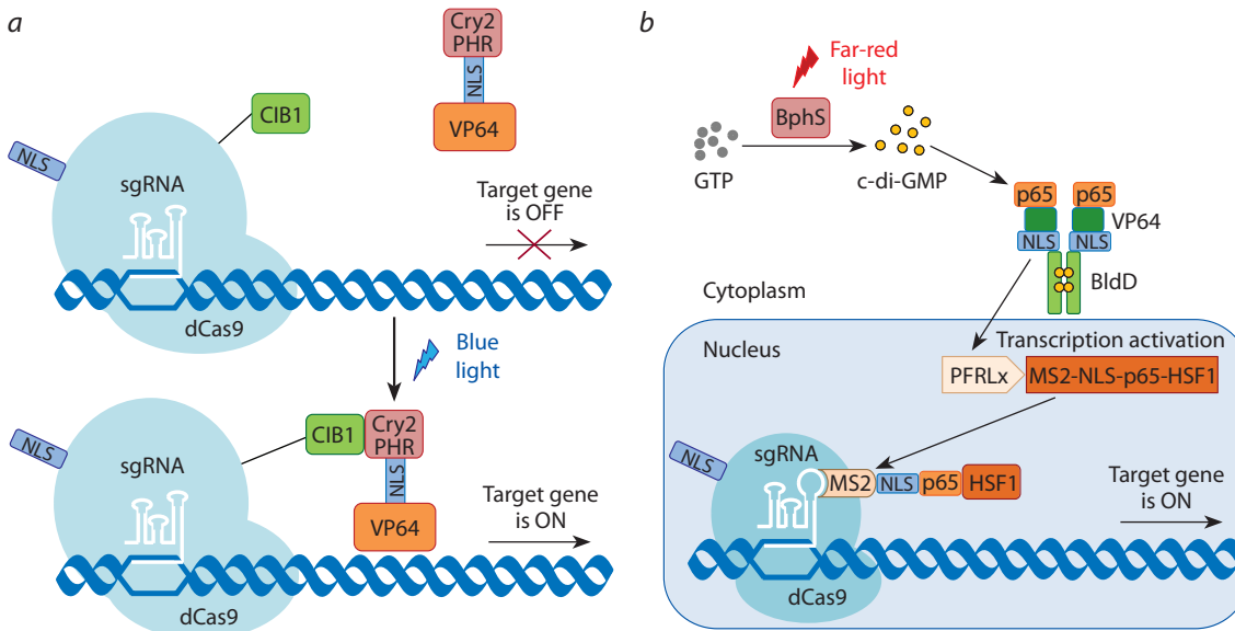
Fig. 3. The principle of the CRISPR/Cas9-based photoactivatable transcription systems.
